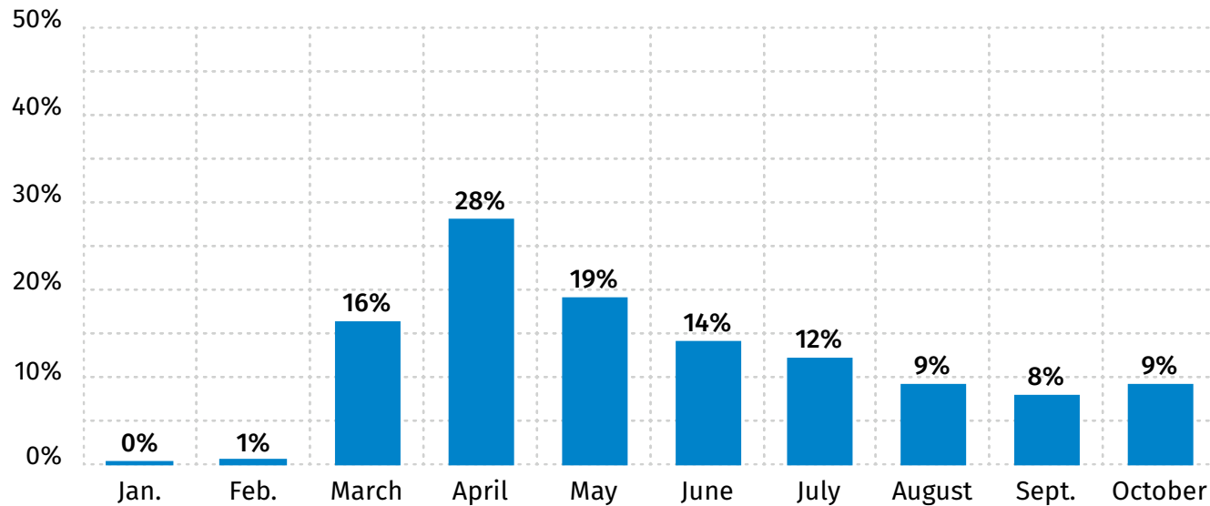
Percentage of COVID-19 Activity Globally
